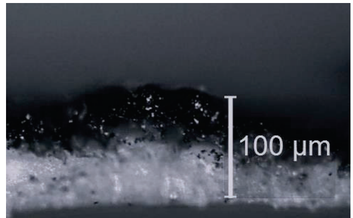
FIGURE 5: A CROSS SECTIONAL MAGNIFIED OPTICAL MICROSCOPE IMAGE OF DEPTH OF THE PYROLIZED PI WITH HATCH DISTANCE OF 25 \mu\text{m} WITH PPD OF 1.
