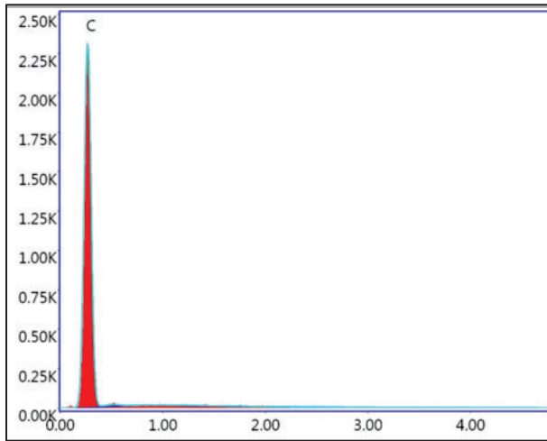
FIGURE 7: EDS GRAPH OF CARBONIZED POLYIMIDE WITH HATCH DISTANCE 25µm AND PPD OF 1.
