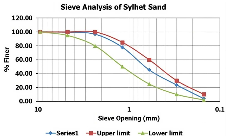
Figure 2. Gradation curve for fine aggregate.
