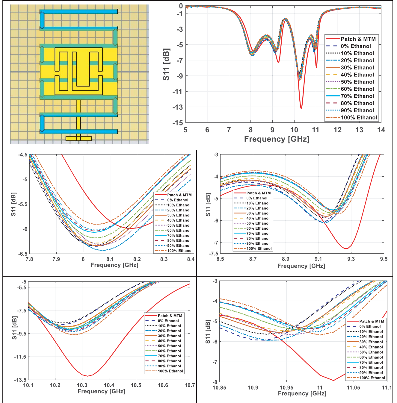
Figure 13. An optimized MTM 8-line fluidic channel sensor system and their sensing responses on different ethanol concentrations.
