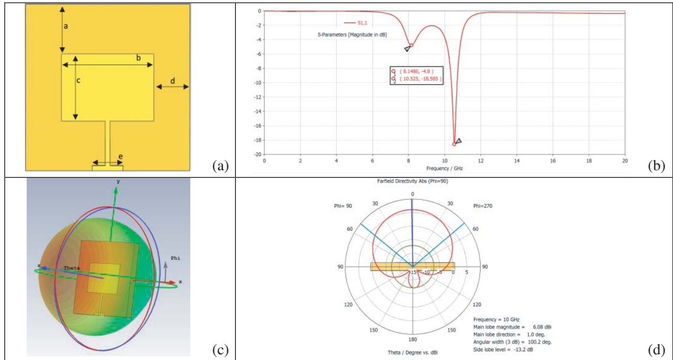
Figure 1. X-band patch antenna and its transmission coefficient and far-field distribution.
