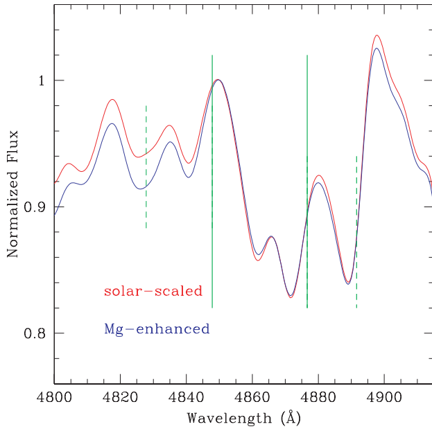
Figure 12. Solar-scaled and Mg-enhanced 12 Gyr integrated spectra near H \beta (4861 Å). Note that the Mg lines make the blue-continuum levels significantly lower, which consequently make the H \beta index strengths weaker as we see in the upper-right panel of Figure 10.
