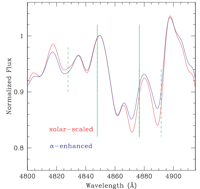
Figure 14. Solar-scaled and the \alpha -enhanced 12 Gyr integrated spectra near H \beta (4861 Å). Note that the \alpha -enhanced spectra at constant Z mostly reflect the Fe depression effect which is the opposite of what is seen in Figure 13 and they affect the H \beta index strengths little as we see in the lower-right panel of Figure 10.
