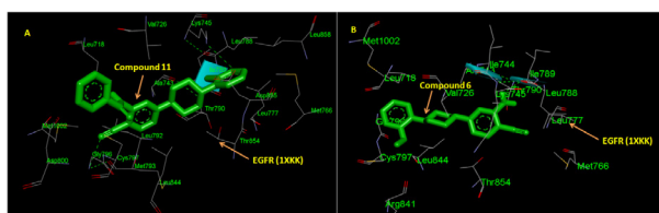
Figure 2: A) Binding pose of Compound 11 and EGFR B) Binding pose of Compound 6 and EGFR.
