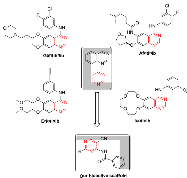
Fig. 1 An amount of clinically approved EGFR-TK inhibitors based on quinazoline and quinoline scaffolds.
