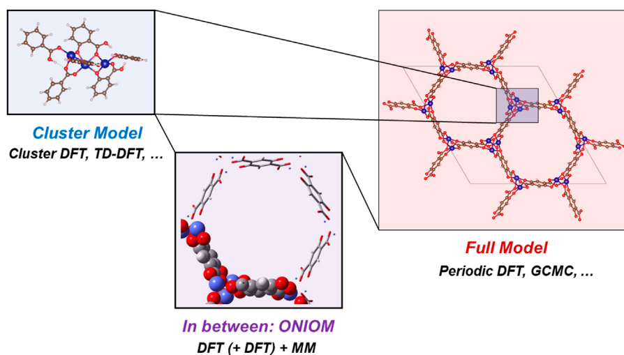
FIGURE 2 Illustration of different levels of models in computational study of MOFs.
