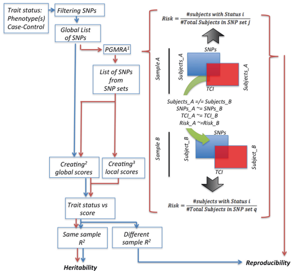
Fig. 1 Flow chart describing the common, as well as the different, roads followed by methods developed to build polygenic scores and the PGMRA method
