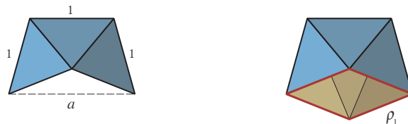
FIGURE 2. Construction of unit rhombus \rho_1 in the proof of Lemma 2.1.
