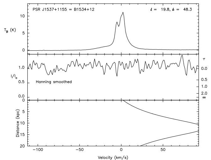
FIG. 10.—Same as Fig. 1, but toward PSR J1537+1155 = B1534+12.
