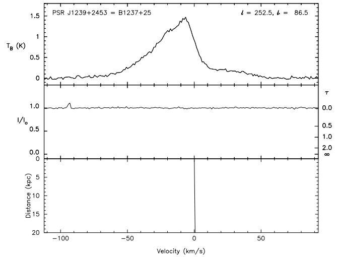
FIG. 9.—Same as Fig. 1, but toward PSR J1239+2453 = B1237+25.
