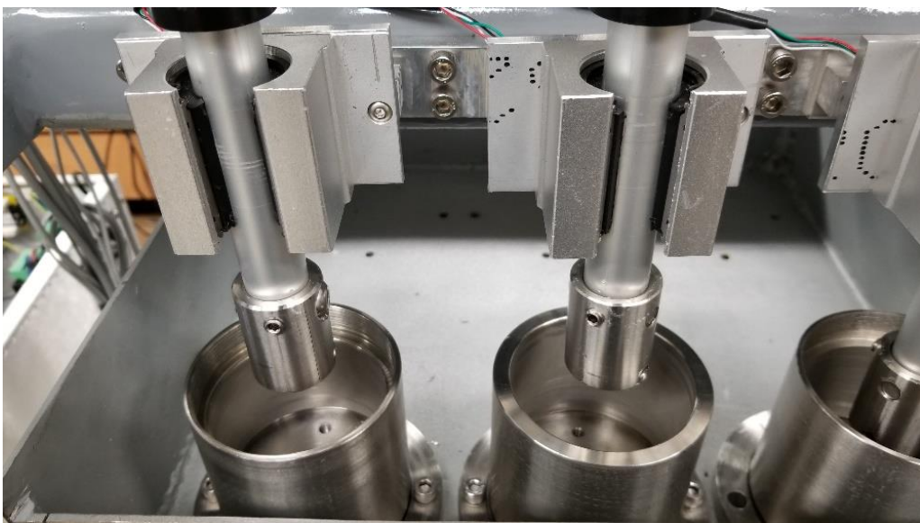
Figure 4.13. – Pin Holder Installed On Each Linear Actuator.
