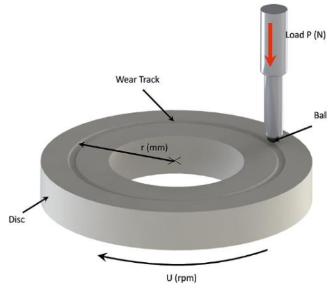
Figure 2.5. – General Schematic Of A Pin On Disk.
