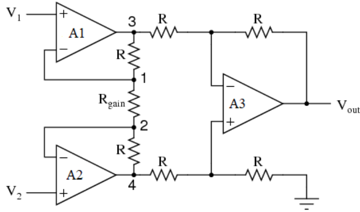
Figure 3.9. – Instrumentation Amplifier.
