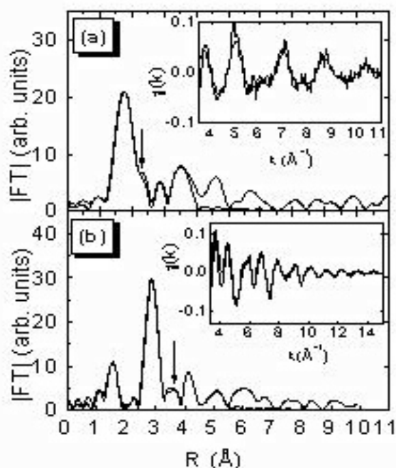
Figure 1 Fourier transform of the \chi(k) spectrum shown in the inset recorded at the (a) N-K-edge and (b) Ga-K-edge. The fitting and the experimental curve are shown in thick and thin solid line, respectively. The arrows indicate the additional paths used for the fitting.
